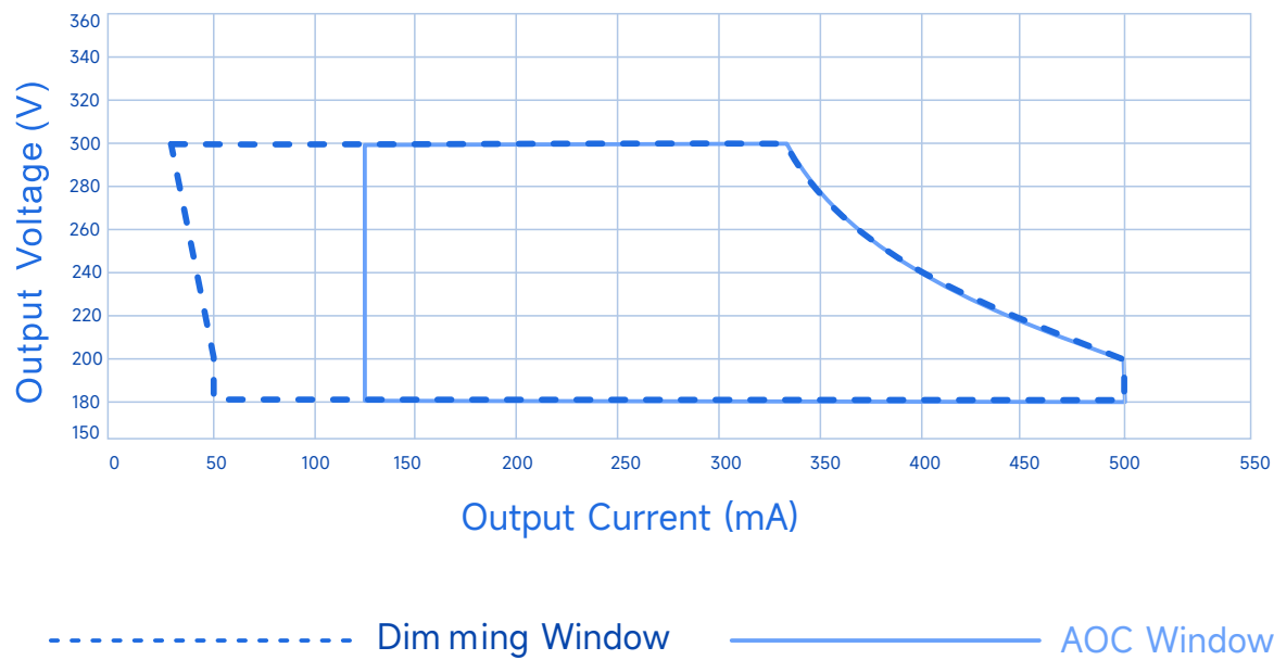
Output Voltage Vs. Output Current(Dim/AOC Window)
